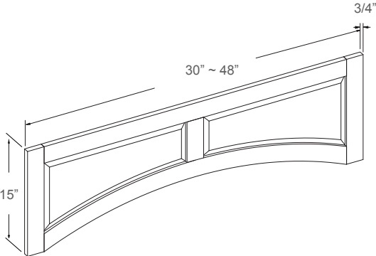
Arch Valance with Raised Panel
